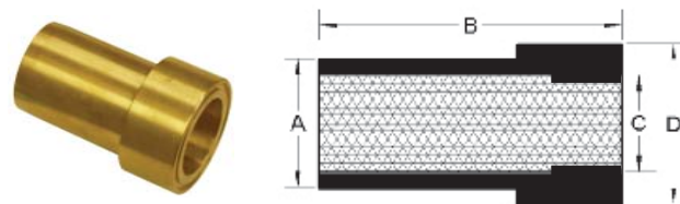
Type 2 Square Shoulder
